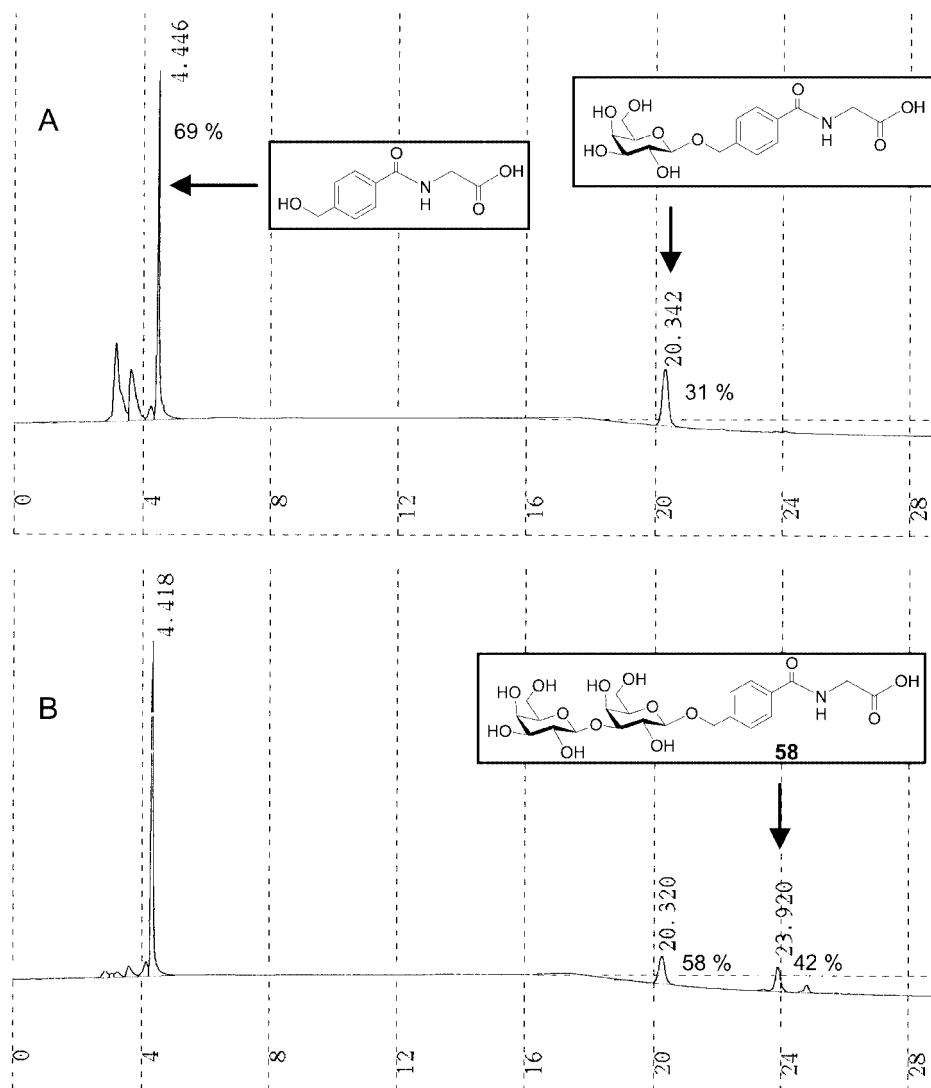
Figure 1. HPLC traces: A) After double coupling of initial sugar to the resin. B) After double coupling of secondary sugar to the resin. The yield was calculated by peak area.
