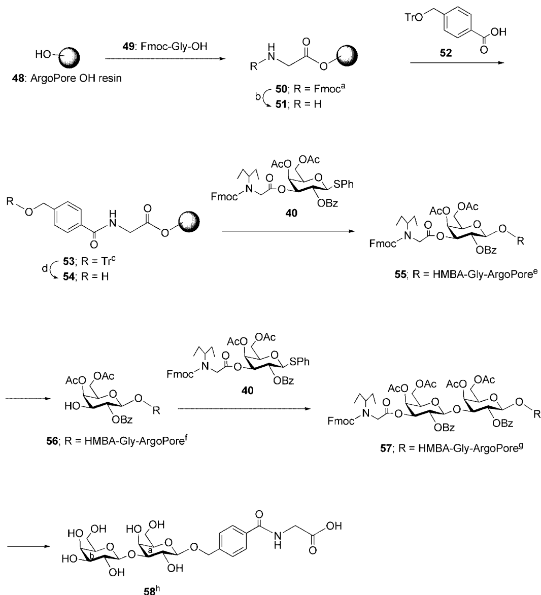
Scheme 7. Reagents and conditions. a 49 , DIC, DMAP, CH 2 Cl 2 , room temp., 7 h, then Ac 2 O, pyr., CH 2 Cl 2 , room temp., 2 h; b 20% piperidine in DMF, room temp., 22 min; c 52 , NEM, TBTU, DMF, room temp., 4 h; d 90% TFA in H 2 O, room temp., 3 h; e 40 , DMTST, CH 2 Cl 2 , room temp., 1 d. This was repeated once more, then Ac 2 O, pyr., CH 2 Cl 2 , room temp., 2 h; f , i , 20% piperidine in DMF, room temp., 22 min, ii), PITC, NMM, DMF, room temp., 2 h; g 40 , DMTST, CH 2 Cl 2 , room temp., 1 d, this was repeated once more; h NaOMe in MeOH, CH 2 Cl 2 , MeOH, room temp., 1 d, then added H 2 O, room temp., 1 d, 4% (8 steps from 50 ).
