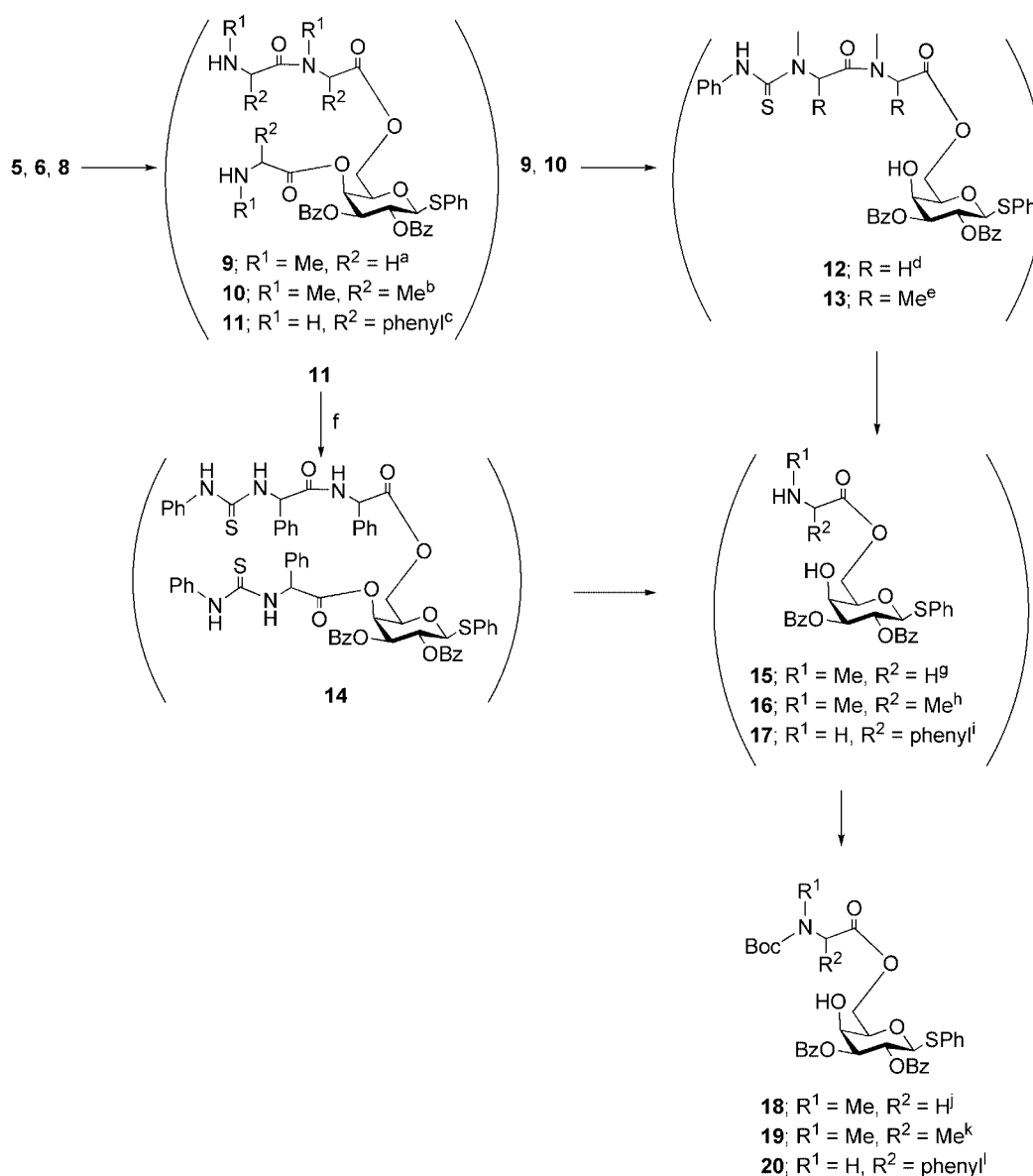
Scheme 2. Reagents and conditions. a 5 , TFA, \text{CH}_2\text{Cl}_2 , room temp., 30 min; b 6 , TFA, \text{CH}_2\text{Cl}_2 , room temp., 30 min; c 8 , TFA, \text{CH}_2\text{Cl}_2 , room temp., 30 min; d 9 , PITC, NMM, DMF, room temp., 30 min; e 10 , PITC, NMM, DMF, room temp., 30 min; f 11 , PITC, NMM, DMF, room temp., 30 min; g 12 , TFA, \text{CH}_2\text{Cl}_2 , room temp., 30 min; h 13 , TFA, \text{CH}_2\text{Cl}_2 , room temp., 30 min; i 14 , TFA, \text{CH}_2\text{Cl}_2 , room temp., 30 min; j 15 , \text{Boc}_2\text{O} , satd. aq. \text{NaHCO}_3 , DMF, room temp., 30 min, 47% (4 steps); k 16 , \text{Boc}_2\text{O} , satd. aq. \text{NaHCO}_3 , DMF, room temp., 30 min, 62% (4 steps); l 17 , \text{Boc}_2\text{O} , satd. aq. \text{NaHCO}_3 , DMF, room temp., 30 min, 69% (4 steps).
