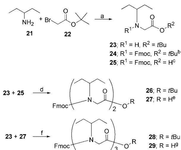
Scheme 3. Reagents and conditions. a THF, room temp., 4 h, 98%; b Fmoc-Cl, 1,4-dioxane/satd. aq. NaHCO 3 , room temp., 2 h, 86%; c 90% formic acid, 40 °C, 7 h, 90%; d DIPEA, PyBroP, DMF, room temp., 30 min, 91%; e 90% formic acid, 50 °C, 3 h, 93%; f DIPEA, PyBroP, DMF, room temp., 30 min, 85%; g 90% formic acid, 50 °C, 2 h, 98%.
