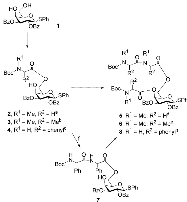
Scheme 1. Reagents and conditions. a 1 , Boc-Sar-OH, cyanuric chloride, pyr., room temp., 1 h, 97%; b 1 , symmetrical anhydride (Boc- N -Me-Ala-OH, DIC, CH 2 Cl 2 , 0 °C, 40 min.), DMAP, DMF, room temp., 1 h, 78%; c 1 , symmetrical anhydride (Boc-Phe-OH, DIC, CH 2 Cl 2 , 0 °C, 40 min.), DMAP, DMF, room temp., 1 h, 94%; d 2 , TFA, CH 2 Cl 2 , room temp., 30 min. ii), symmetrical anhydride (Boc-Sar-OH, DIC, CH 2 Cl 2 , 0 °C, 40 min.), DMAP, DMF, room temp., 1 h, 73%; e 3 , TFA, CH 2 Cl 2 , room temp., 30 min. ii), symmetrical anhydride (Boc- N -Me-Ala-OH, DIC, CH 2 Cl 2 , 0 °C, 40 min.), DMAP, DMF, room temp., 1 h, 75%; f 4 , TFA, CH 2 Cl 2 , room temp., 30 min. ii), symmetrical anhydride (Boc-Phe-OH, DIC, CH 2 Cl 2 , 0 °C, 40 min.), DMAP, DMF, room temp., 1 h, 92%; g 7 , symmetrical anhydride (Boc-Phe-OH, DIC, CH 2 Cl 2 , 0 °C, 40 min.), DMAP, pyr., 50 °C, 5 h, 68%.
